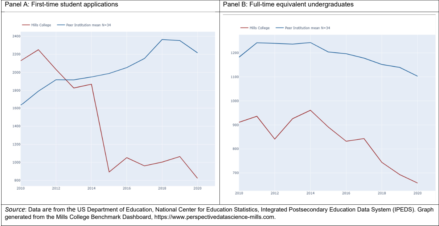
FIGURE 7 Mills College's undergraduate enrollment problem
